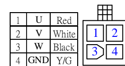
Motor Connection
