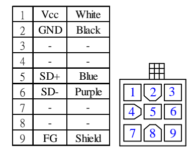
Encoder Connection
